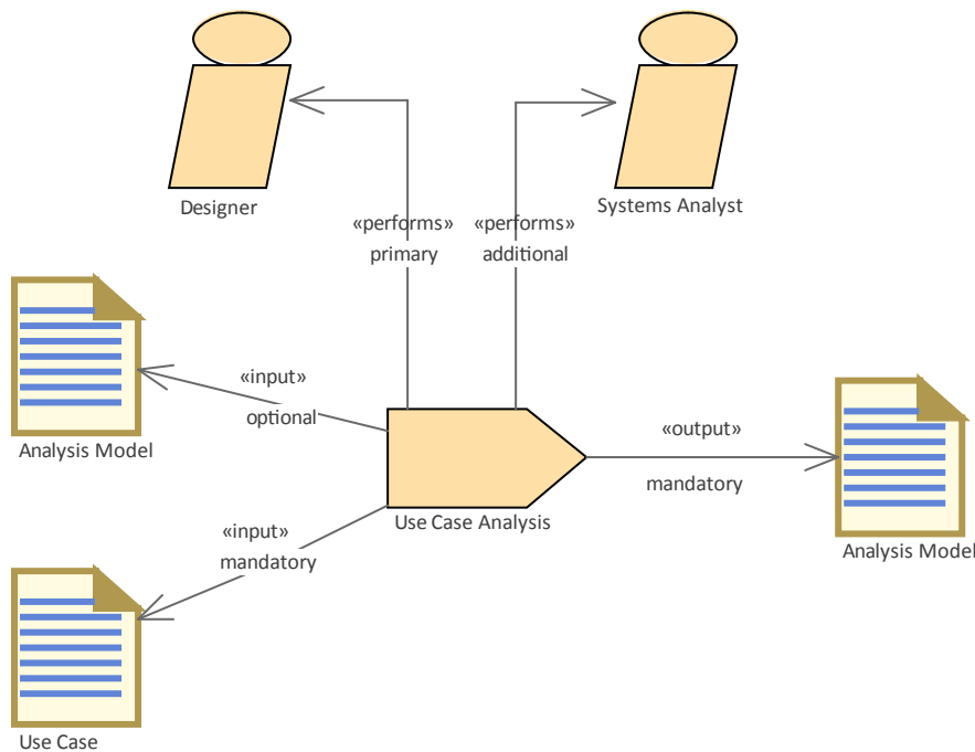
SPEM model showing the key performers and input and output parameters for a Use Case Analysis task.
