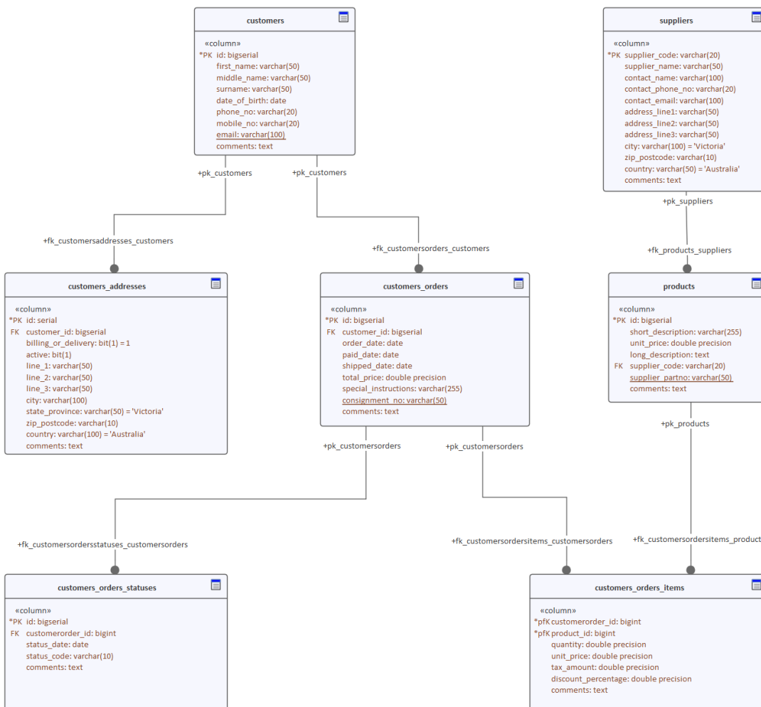
Data modeling diagram with suppressed operation
